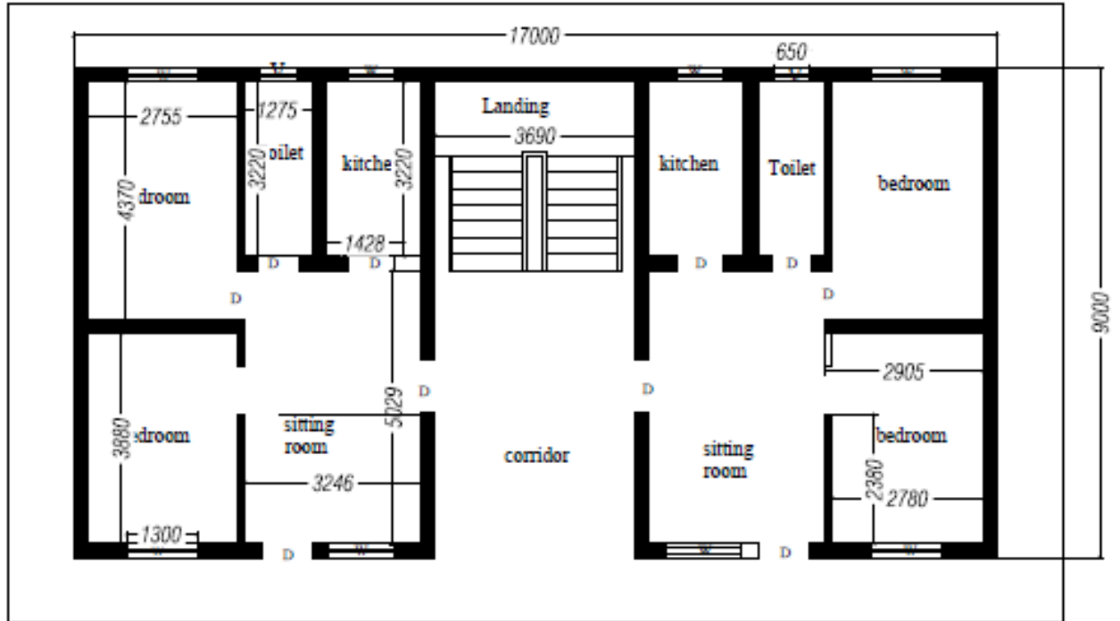
Layout plan of four unit staff quarter(F)
