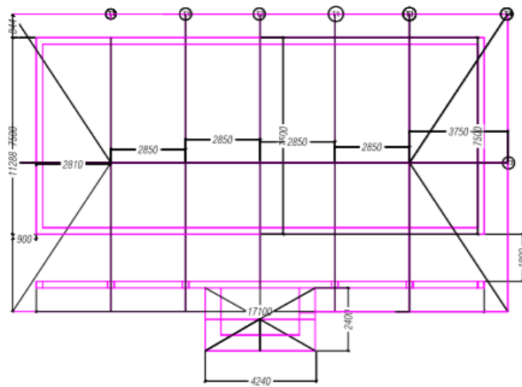
Roof layout plan for early learning centre
